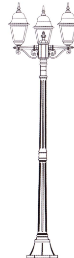
79908B S M L h=1900 2045 1881
