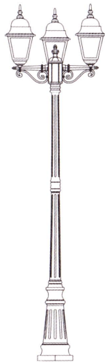
79909B h=2385
