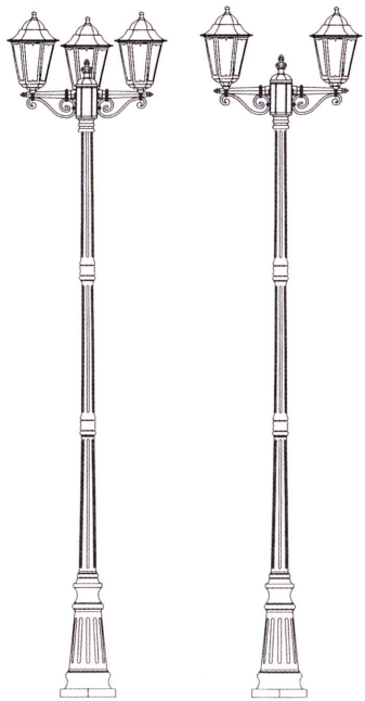
79810B S M L h=2710 2770 2855 h=2990 3050 3135 79810A S M L h=2710 2770 2855 h=2990 3050 3135
