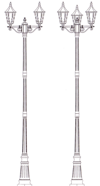
79710A S M L h=2710 2770 2855 h=2990 3050 3135 79710B S M L h=2710 2770 2855 h=2990 3050 3135
